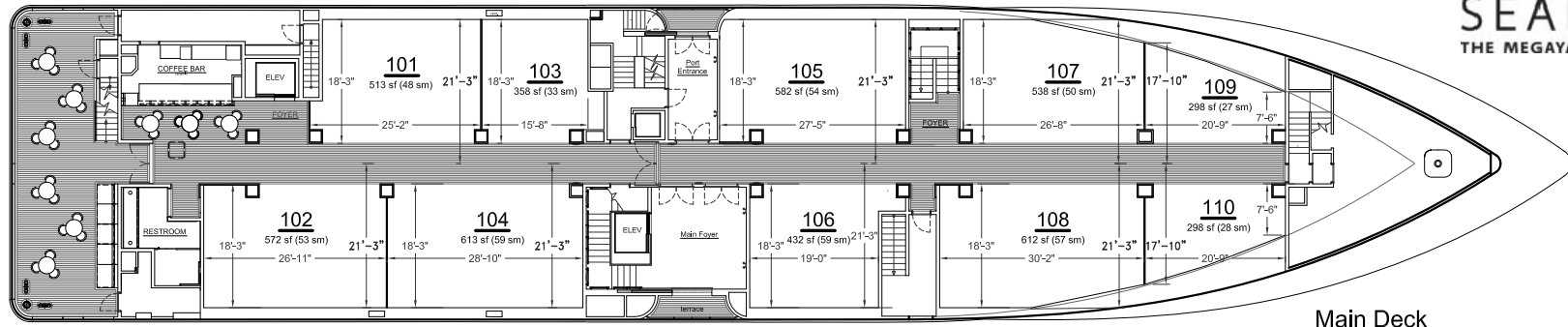
Main Deck
